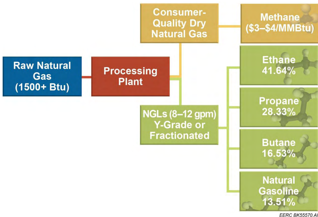
Figure 3. Natural gas processing (NGLs are natural gas liquids).
