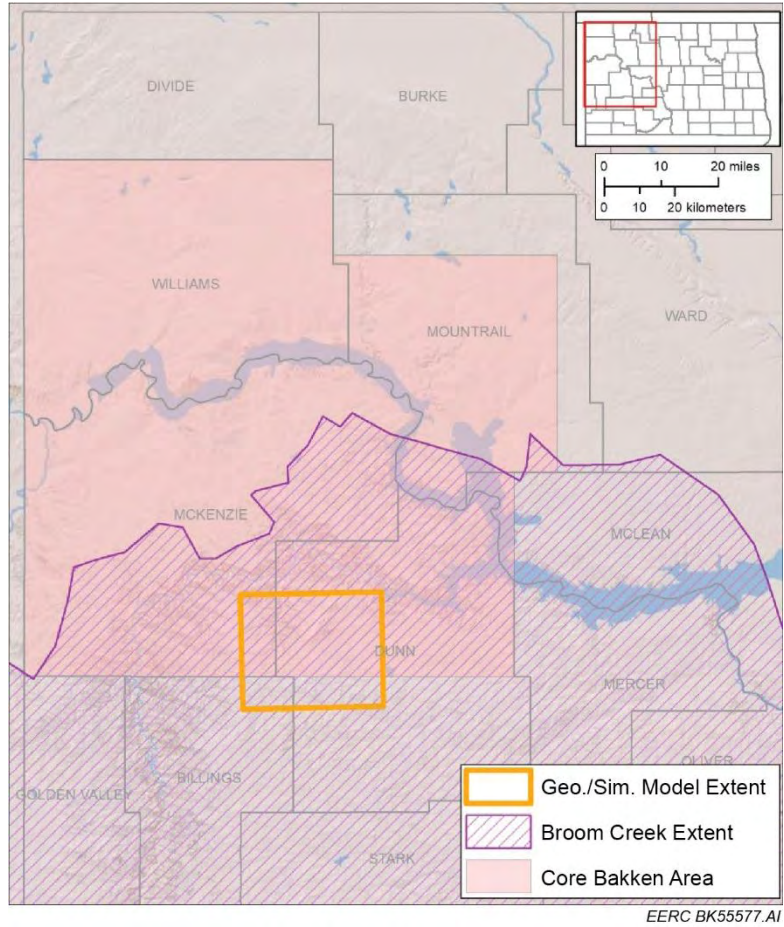
Figure A-1. Map showing the location of the geologic and simulation model.
