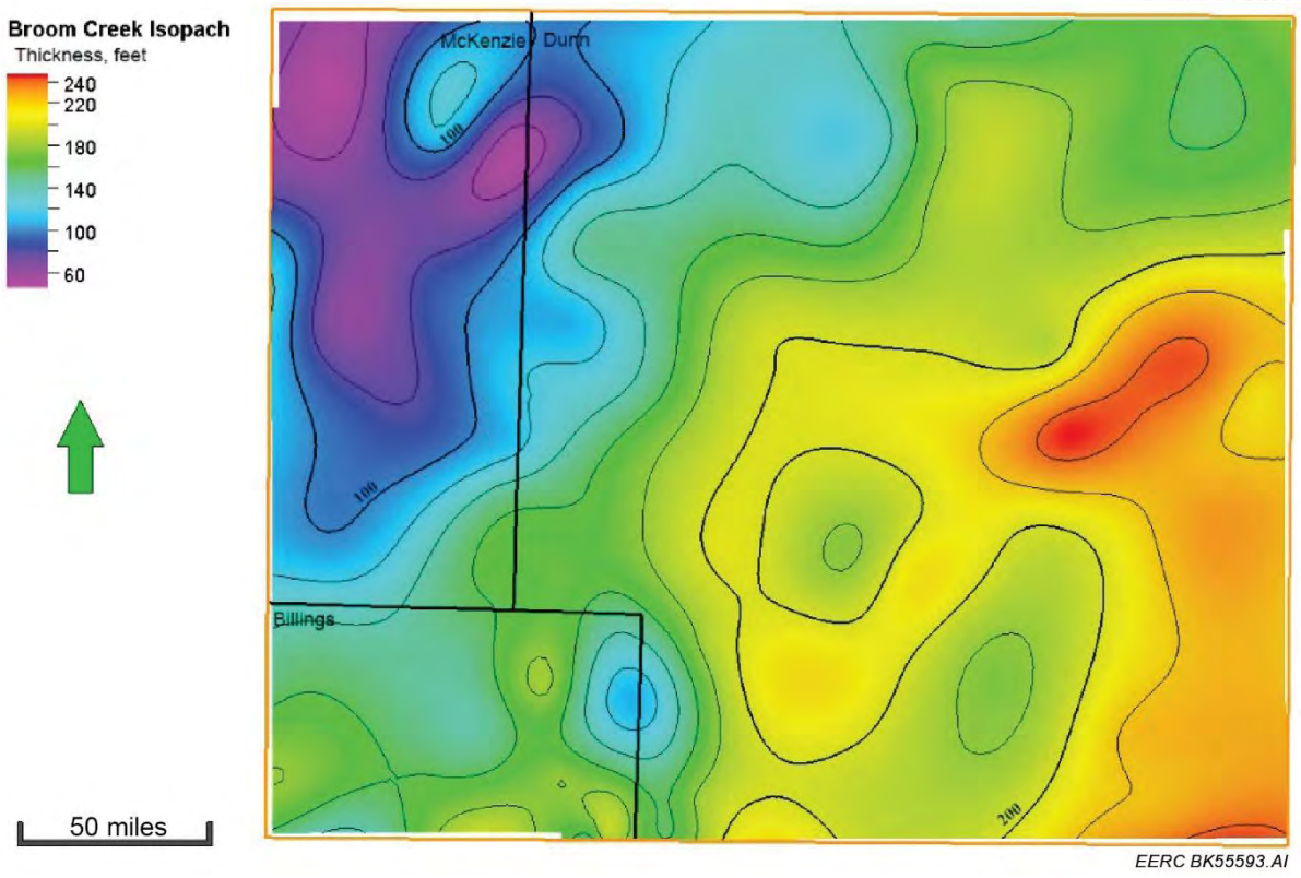
Figure A-2. Maps of the Broom Creek Formation within the modeled area. Top: Broom Creek Formation structure contour (datum is mean sea level, contour interval = 20 ft), bottom: Broom Creek Formation isopach (contour interval = 20 ft).
