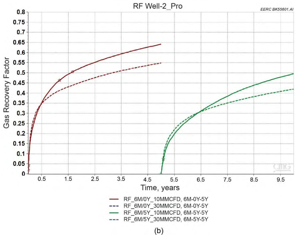
Figure A-10. Well 1 (a) and Well 2 (b) simulated gas recovery factor for 6-month injection, Cases 2-5.
