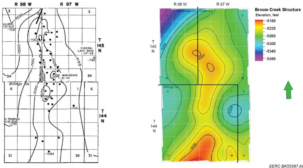
Figure 15. Little Knife Field: (left) structural contour map of the Mission Canyon top (Wittstrom and Hagemier, 1978) and (right) structure contour map of the Broom Creek top.
