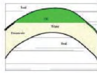
Anticline
