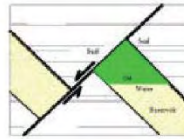
Fault
