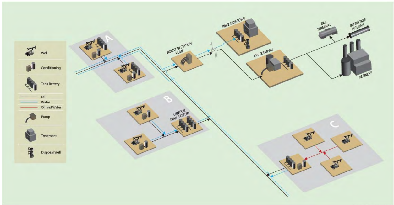
Figure 2. Example gathering infrastructure. Configuration A represents well pumps, conditioning equipment, and tankage on a well pad. Alternate Configuration B represents well pumps and conditioning on the well pad, with fluids stored on a separate central tank battery. Configuration C represents only well pumps on the wellsite, with fluid conditioning and tankage on a centralized conditioning and storage location.
