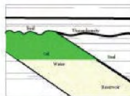
Unconformity
