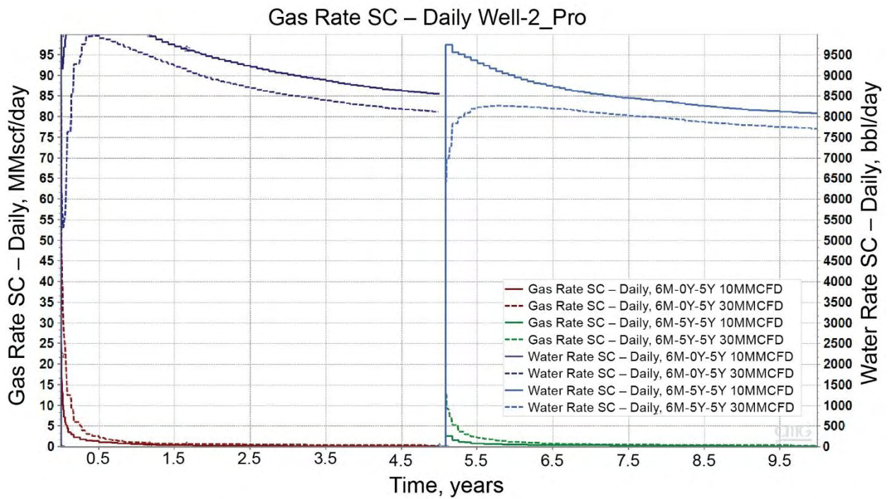
Figure A-11. Well 1 (a) and Well 2 (b) simulated gas/water rate for 6-month injection, Cases 2–5.
