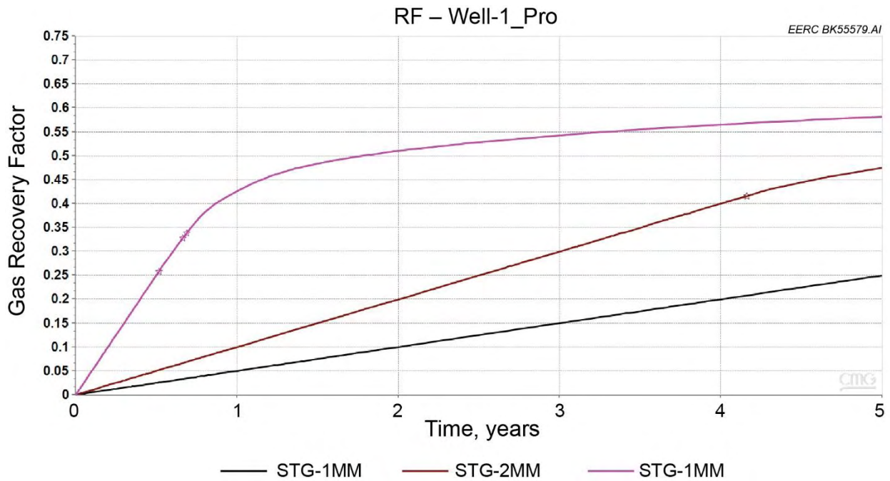
Figure 9. Gas recovery factor for Cases 22–24.
