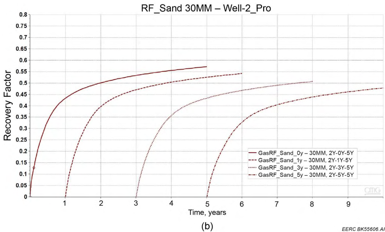
Figure A-14. Well 1 (a) and Well 2 (b) gas recovery factor for 2 years of injection followed by varying shut-in periods and subsequent production, Cases 10–13, 30 MMscf/day injection.
