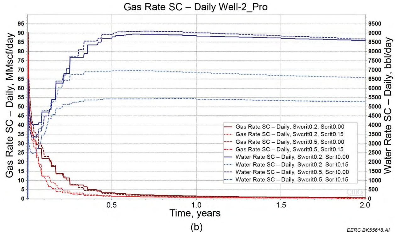
Figure A-22. Well 1 (a) and Well 2 (b) water and gas production rate for Cases 18–21 (injection rate of 10 MMscf/day for 2 years; immediate recovery).
